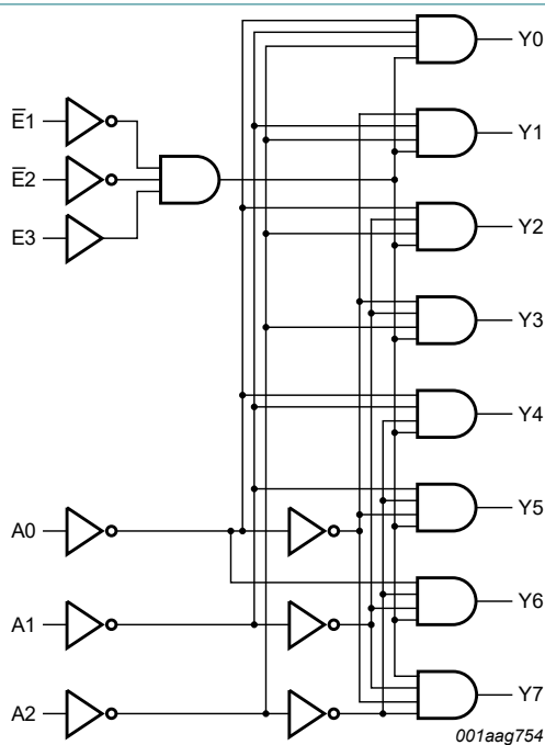
Fig. 2. Functional diagram
