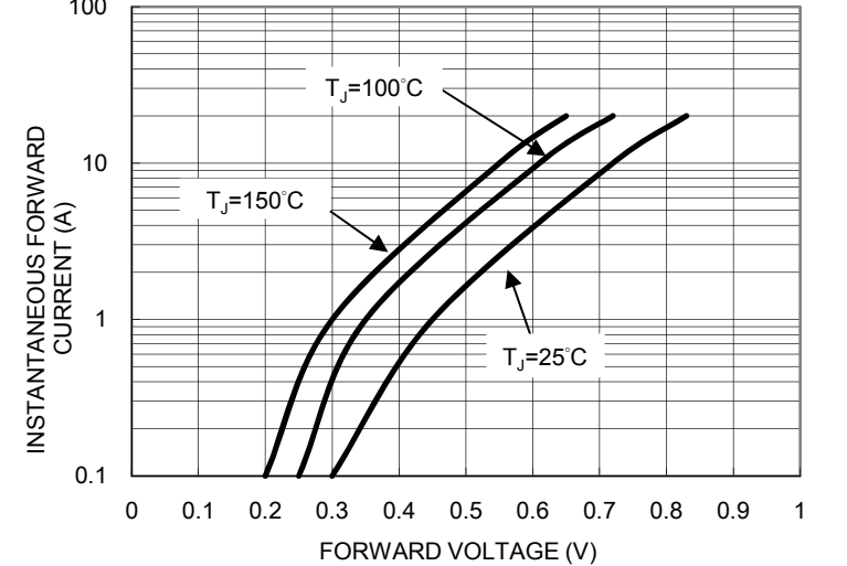
FIG. 3 TYPICAL FORWARD CHARACTERISTICS PER LEG
