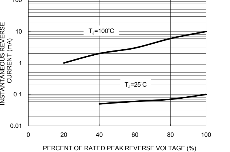
FIG. 4 TYPICAL REVERSE CHARACTERISTICS PER LEG
