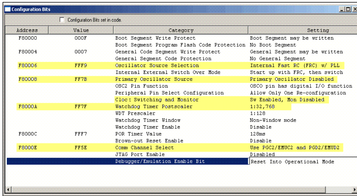
FIGURE 3-14: CONFIGURATION SETTINGS
