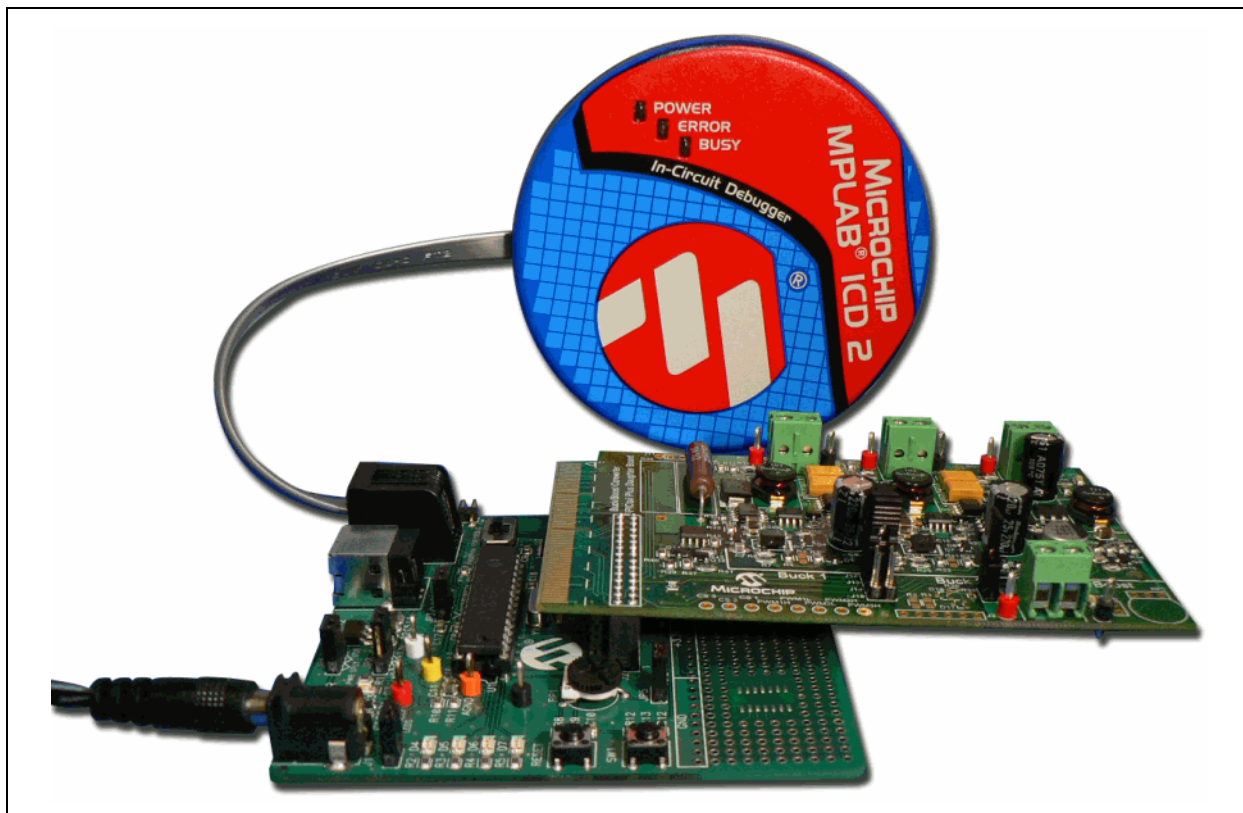
FIGURE 3-15: DAUGHTER BOARD CONNECTED TO MPLAB® ICD 2 IN-CIRCUIT DEBUGGER
