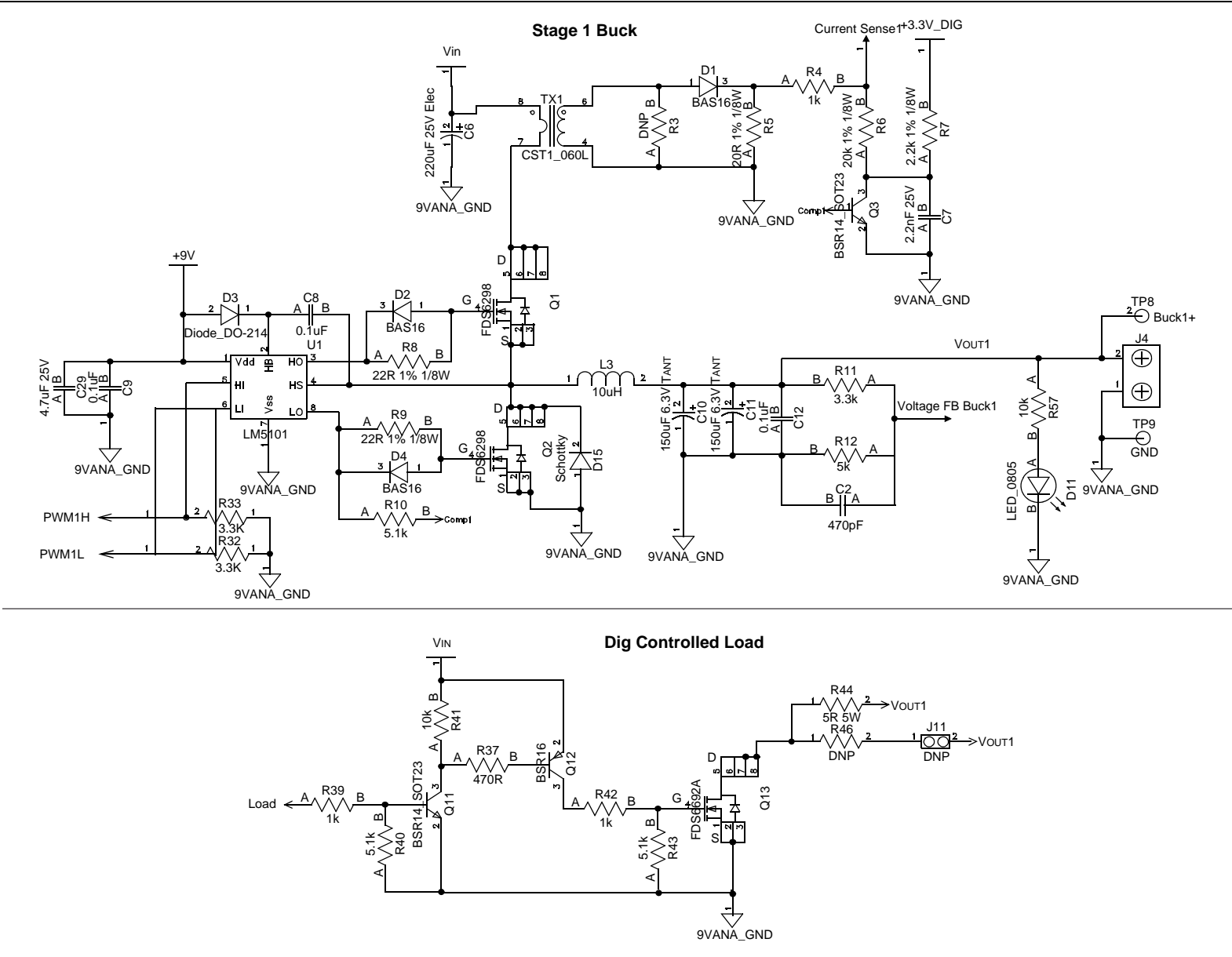
FIGURE A-2: DAUGHTER BOARD SCHEMATIC 1 OF 5
