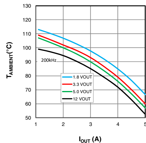
Figure 28: XR76205, V_{IN}=24\text{V}
