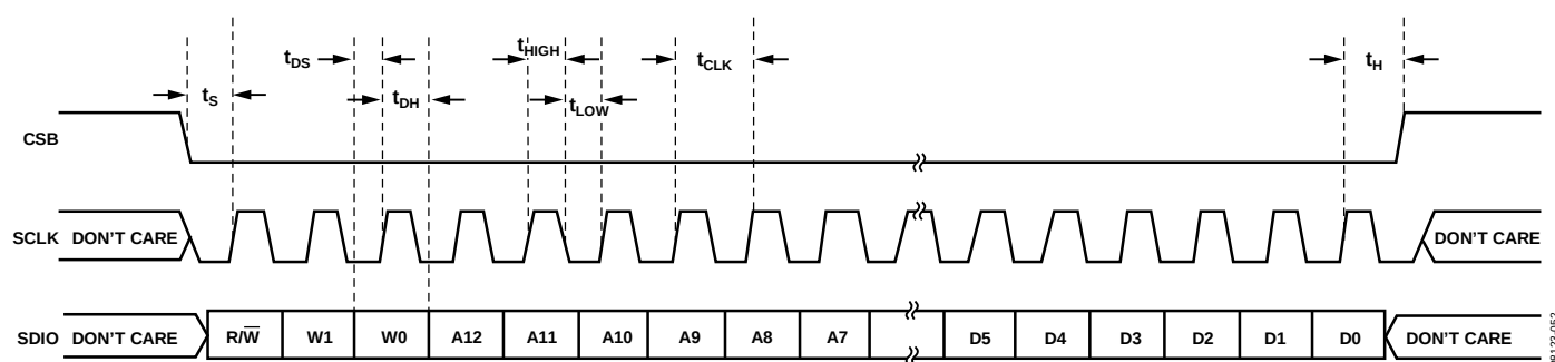
Figure 84. Serial Port Interface Timing Diagram
