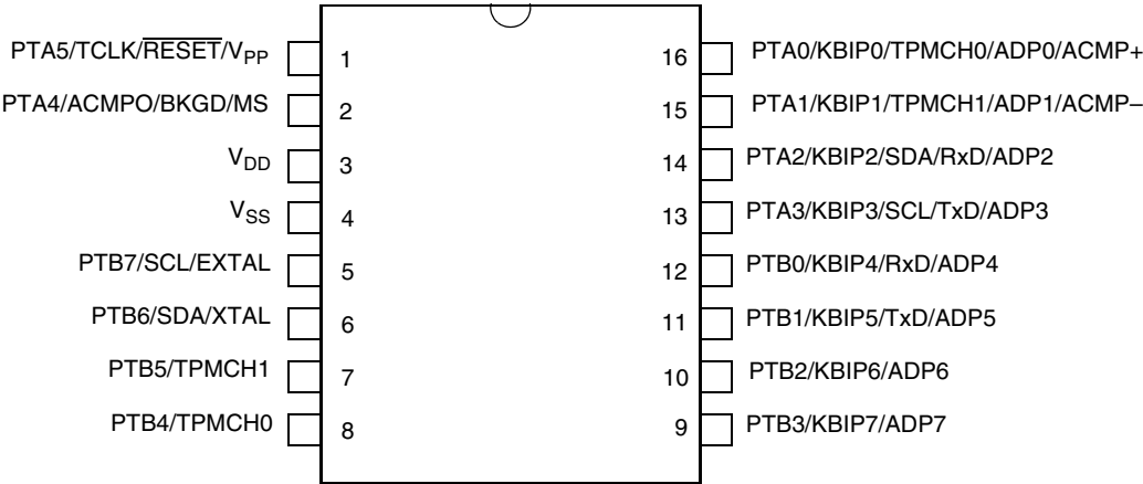
Figure 4. MC9RS08KB12 Series 16-Pin SOIC NB/TSSOP Package
