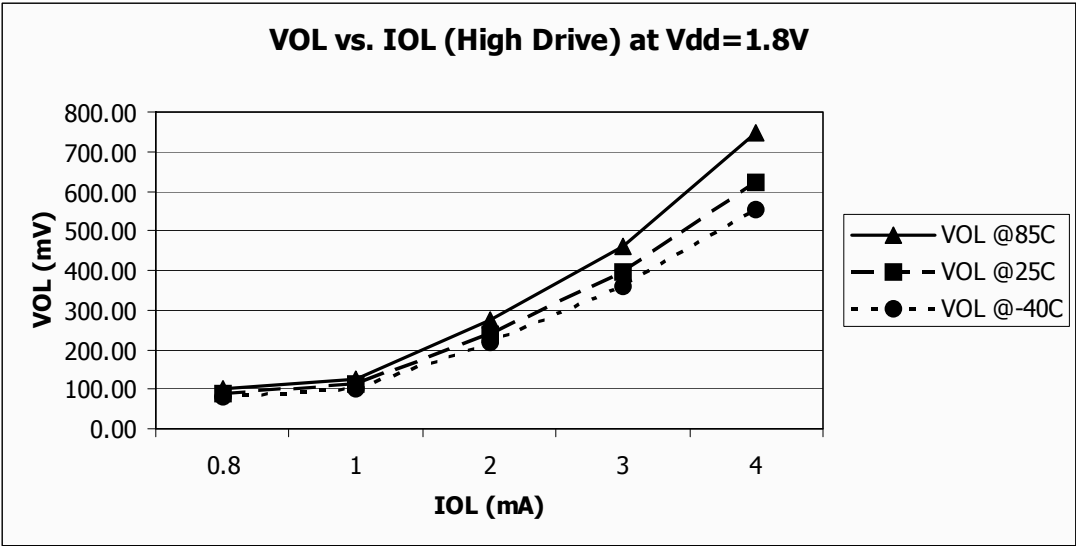
Figure 16. Typical V_{OL} vs. I_{OL} V_{DD} = 1.8\text{ V} (High Drive)
