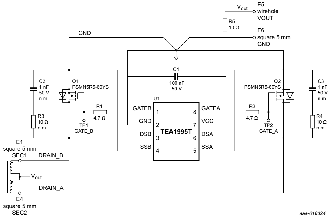
Fig 8. TEA1995DB1295 demo board schematic
