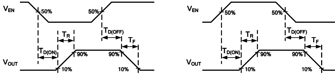
Figure 1. Voltage Waveforms: AP2301A (left), AP2311A (right)
