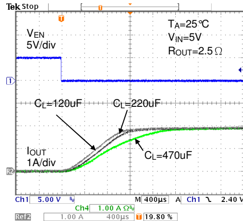
Inrush Current
