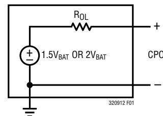
Figure 1. Charge Pump Thevenin Equivalent Open-Loop Circuit
