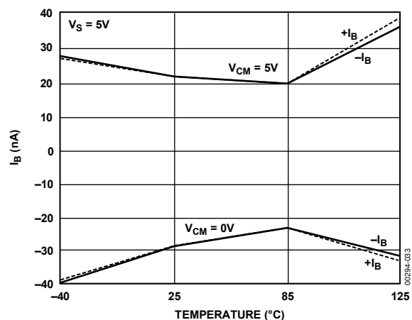
Figure 28. Input Bias Current vs. Temperature, V_S = 5V
