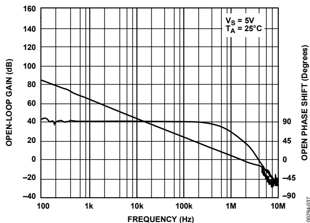
Figure 32. Open-Loop Gain and Phase vs. Frequency, V_S = 5\text{ V}
