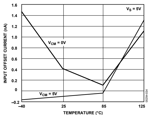
Figure 29. Input Offset Current vs. Temperature, V_S = 5V
