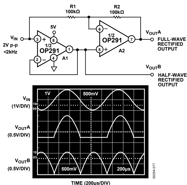
Figure 73. Single-Supply, Half-Wave, and Full-Wave Rectifiers Using an OP291
