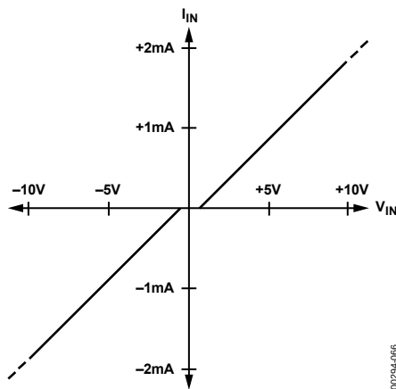
Figure 62. Input Overvoltage Characteristics
