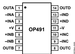
Figure 5. 14-Lead TSSOP
