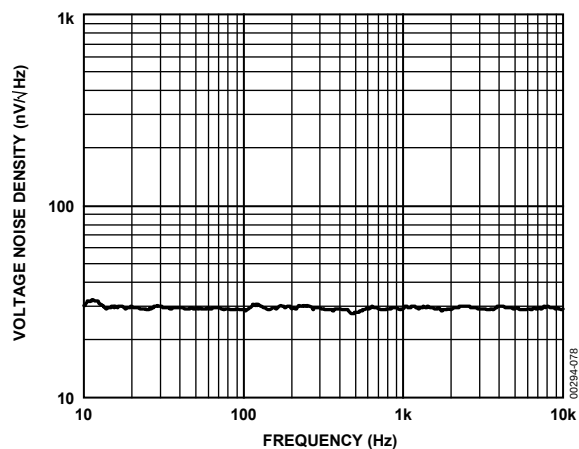
Figure 58. Voltage Noise Density, V_S = 3V
