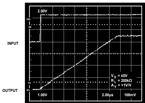
Figure 60. Large Signal Transient Response, V_S = \pm 5V
