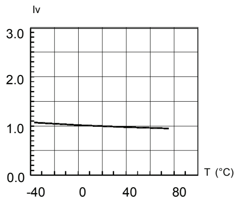
Fig. 6 Relative Luminous Intensity vs. Temperature
