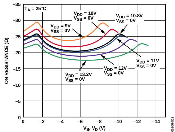
Figure 8. R_{ON} as a Function of V_S , V_D (Single Supply)
