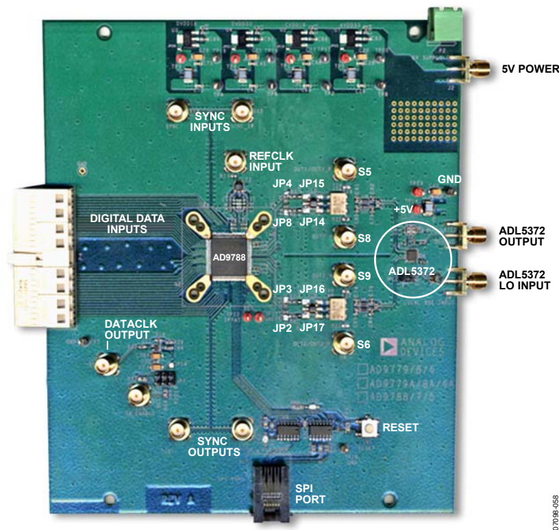
Figure 79. Evaluation Board
