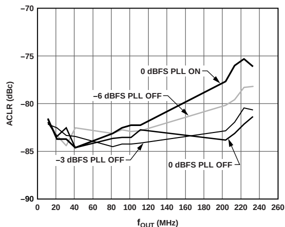
Figure 18. AD9788 ACLR for Third Adjacent Band WCDMA, 4× Interpolation, f_{DATA} = 122.88 MSPS, NCO Translates Baseband Signal to IF
