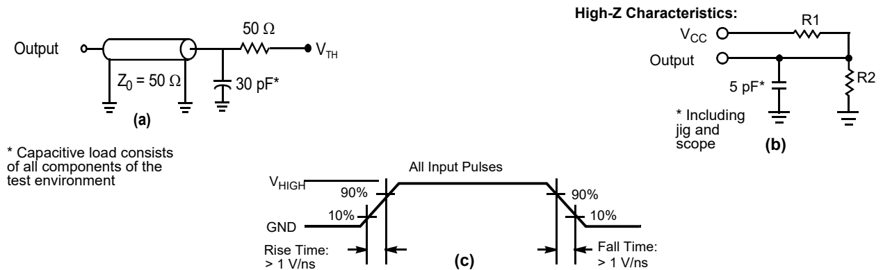
Figure 4. AC Test Loads and Waveforms [12]
