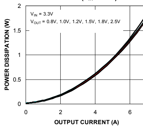
IC Power Dissipation vs. Output Current ( V_{IN} = 3.3V )
