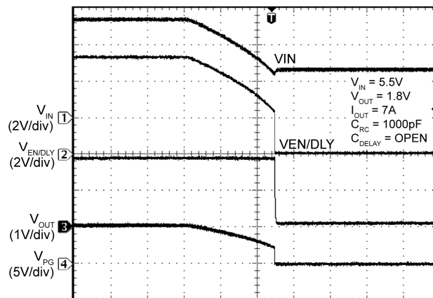
V_{IN} Turn-Off
