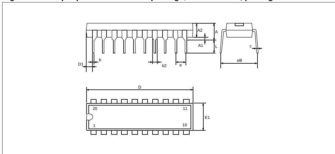
Figure 95. 20-pin plastic dual in-line package, 300-mil width, package outline
