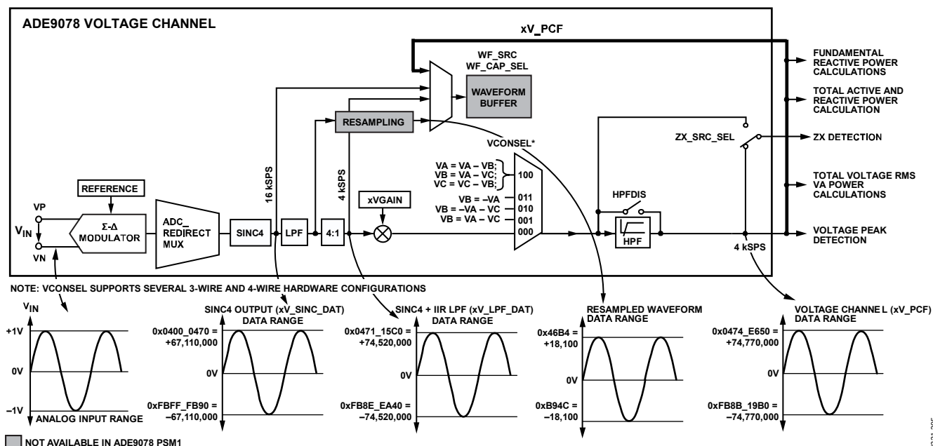
Figure 105. Voltage Channel Datapath
