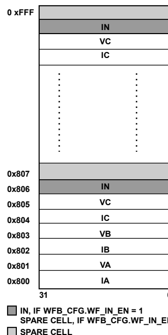
Figure 107. Fixed Data Rate Waveform Sample Storage
