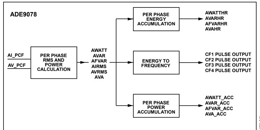
Figure 53. Per Phase Power and Energy Calculations from xI\_PCF and xV\_PCF Waveforms
