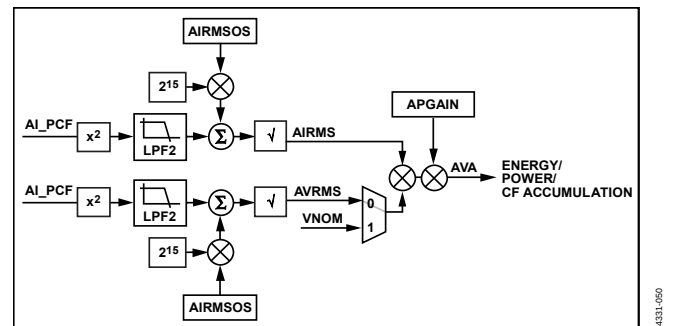
Figure 58. Total Apparent Power (AVA) Calculation
