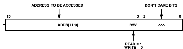
Figure 99. Command Header, CMD_HDR, Bits[15:0]
