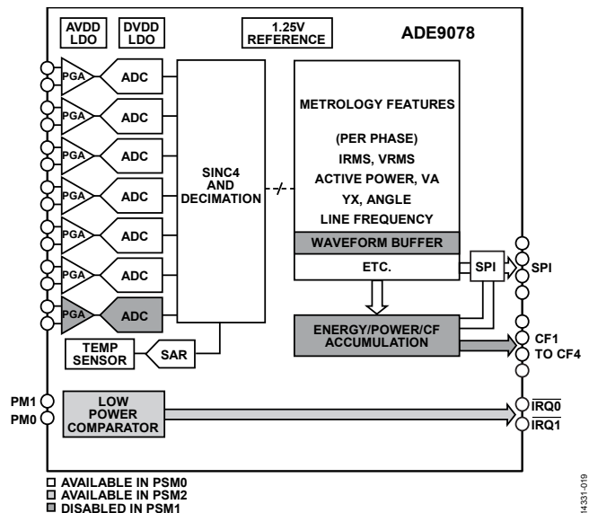
Figure 38. Functions Available in PSM1 and PSM2
