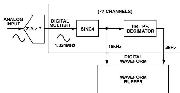
Figure 35. Datapath Following ADC Stage
