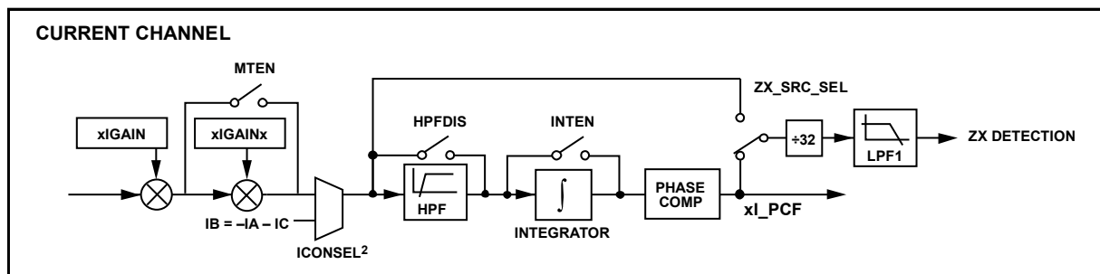
Figure 69. Voltage and Current Channel Signal Chain Preceding Zero-Crossing Detection
