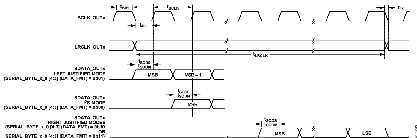
Figure 5. Serial Output Port Timing Specifications
