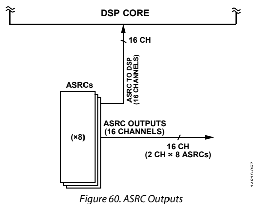
Figure 60. ASRC Outputs
