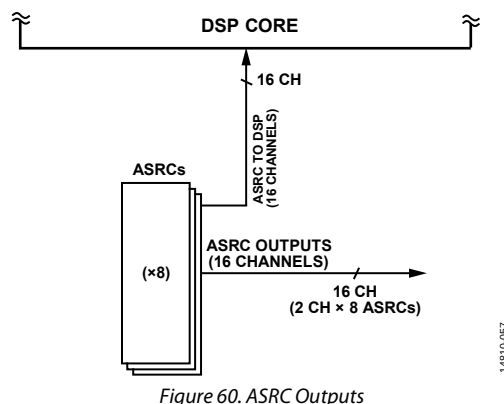
Figure 60. ASRC Outputs
