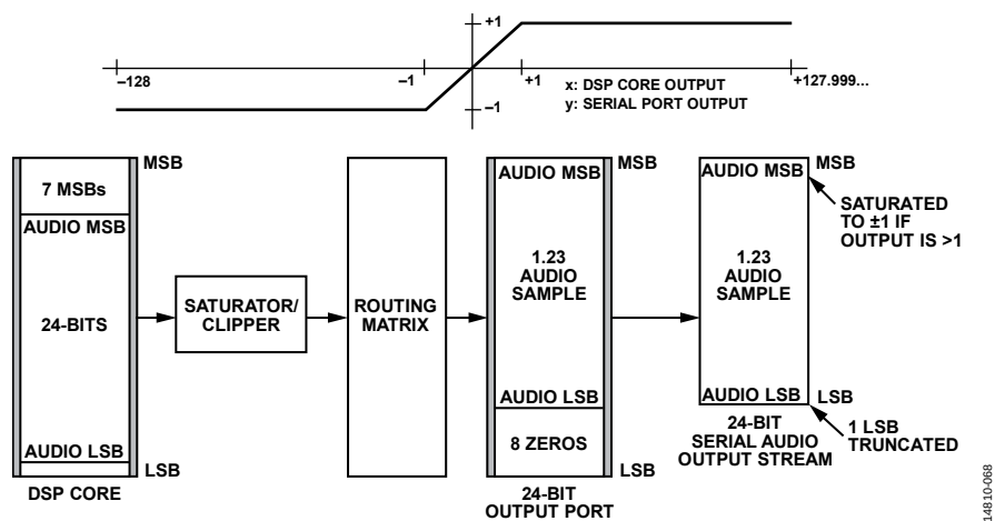
Figure 70. 24-Bit Serial Output Example
