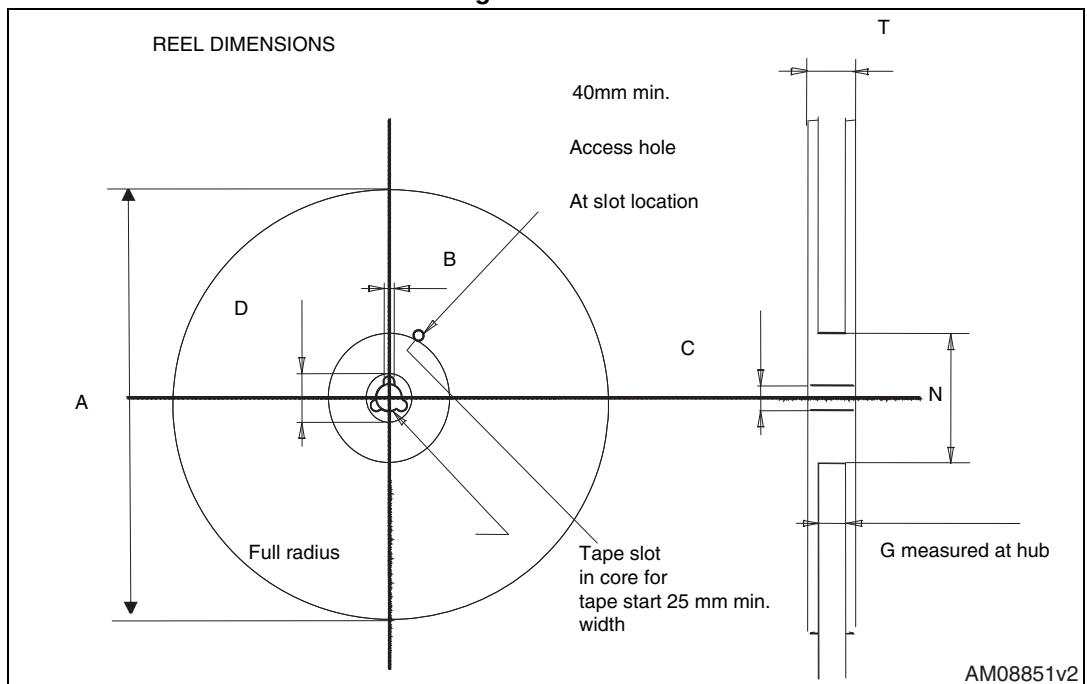
Figure 38. Reel
