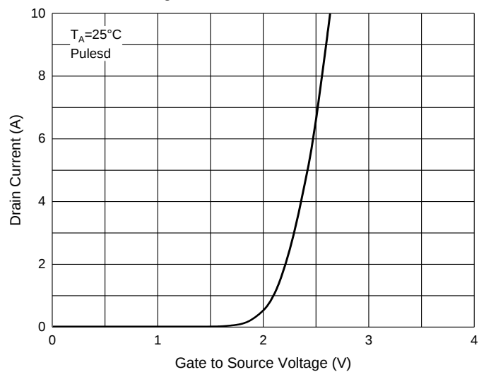
Fig. 2 - Transfer Characteristics
