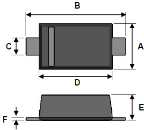
SOD-523F
