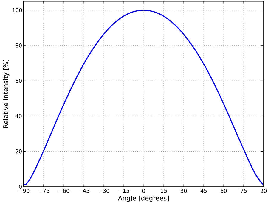
Figure 5. Typical radiation pattern for LUXEON 3014 with FreshFocus Technology at 60mA, T_j=25^{\circ}\text{C} .
