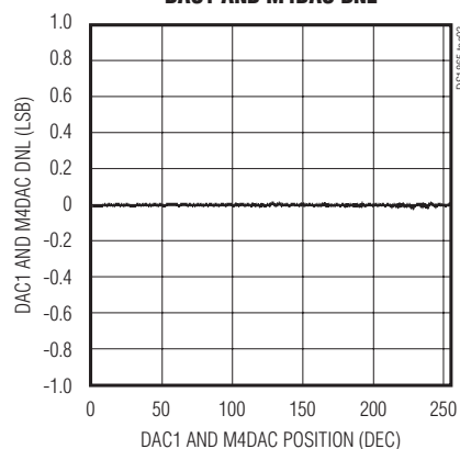
DAC1 AND M4DAC DNL
