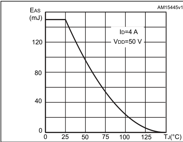
Figure 18. Maximum avalanche energy vs temperature
