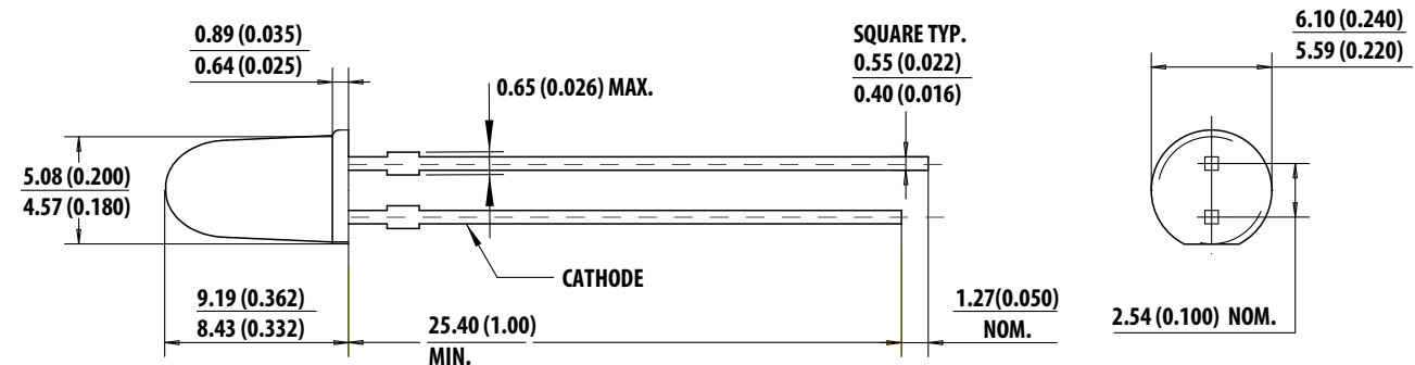
A - HLMP-4700, -4719, -4740
