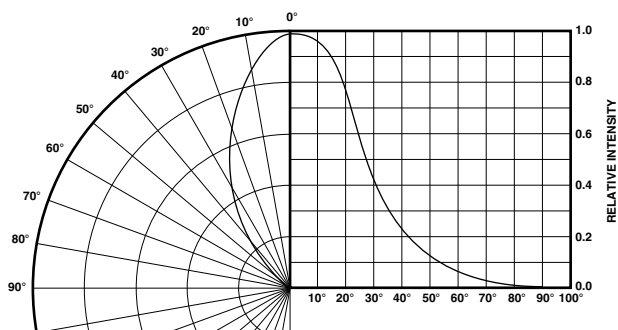
Figure 4. Relative luminous intensity vs. angular displacement for T-1 3/4 lamp.
