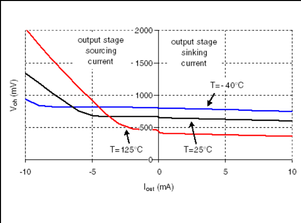
Figure 8. Output stage high-state saturation voltage versus output current ( V_{sense} = +1\text{ V} )
