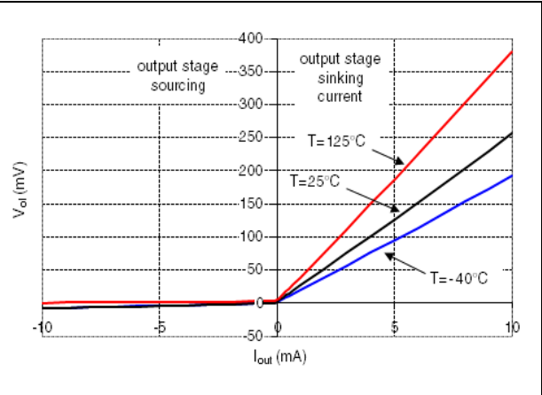
Figure 7. Output stage low-state saturation voltage versus output current ( V_{sense} = -1\text{ V} )
