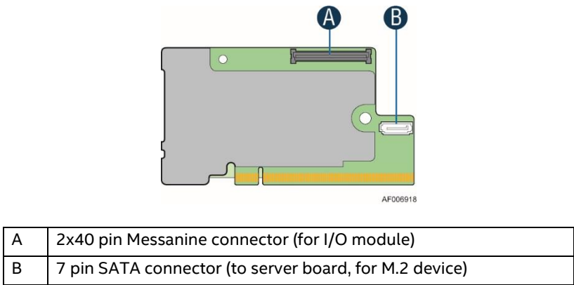
Figure 24. AXXKPTPM2IOM I/O Module Carrier Connectors
