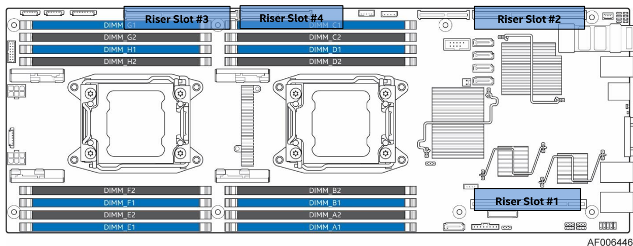
Figure 38. Server Board Riser Slots (S2600TPFR)
