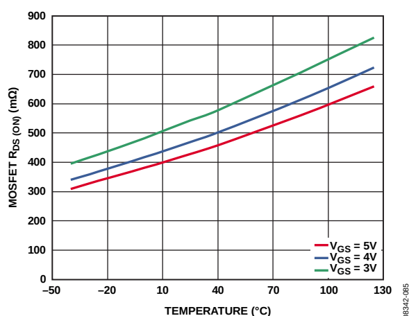
Figure 23. MOSFET R_{\text{DS(ON)}} vs. Temperature (Pin-to-Pin Measurements)
