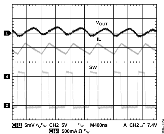
Figure 26. Steady State at Heavy Load, f_{\text{SW}} = 1.4\text{ MHz} , I_{\text{OUT}} = 1\text{ A}
