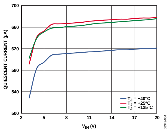
Figure 22. Quiescent Current vs. V_{\text{IN}}
