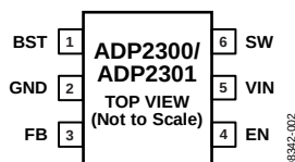
Figure 3. Pin Configuration
