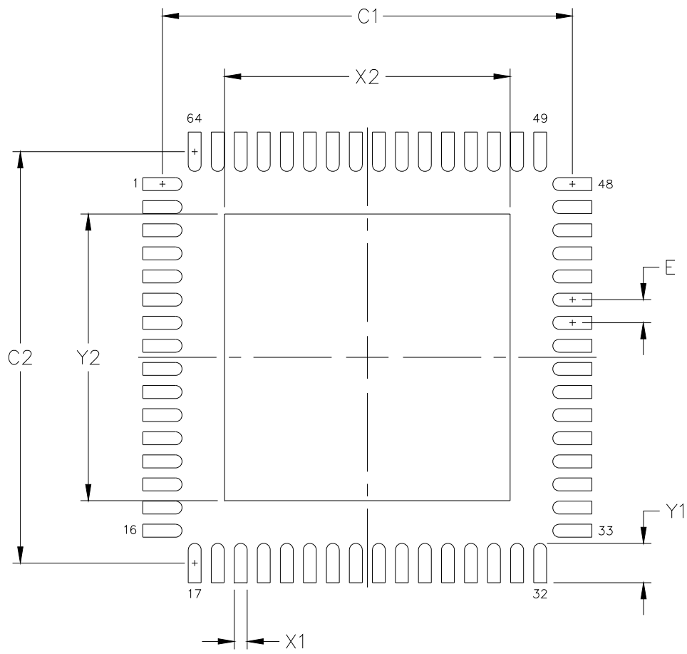
Figure 14. Land Pattern
