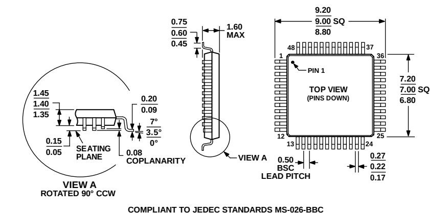
Figure 35. 48-Lead Low Profile Quad Flat Package [LQFP] (ST-48) Dimensions shown in millimeters
