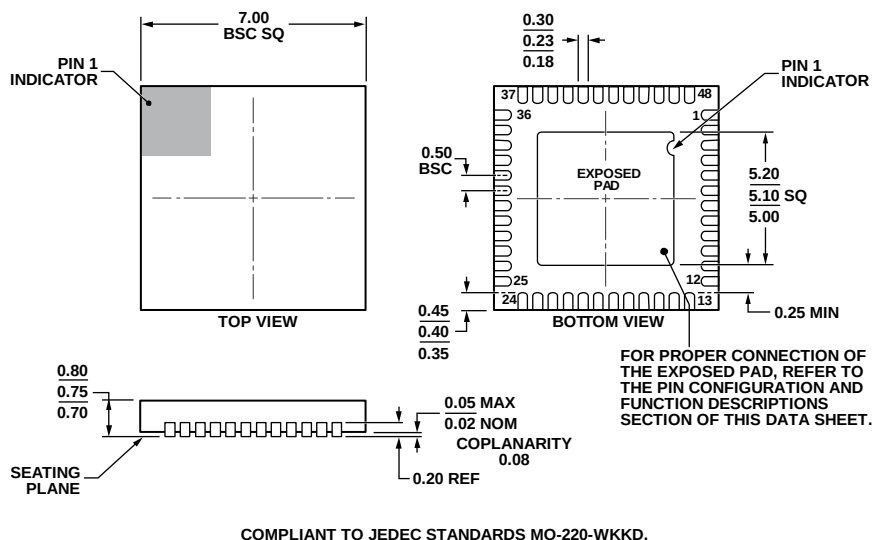
Figure 36. 48-Lead Lead Frame Chip Scale Package [LFCSP] 7 mm × 7 mm Body and 0.75 mm Package Height (CP-48-4) Dimensions shown in millimeters
