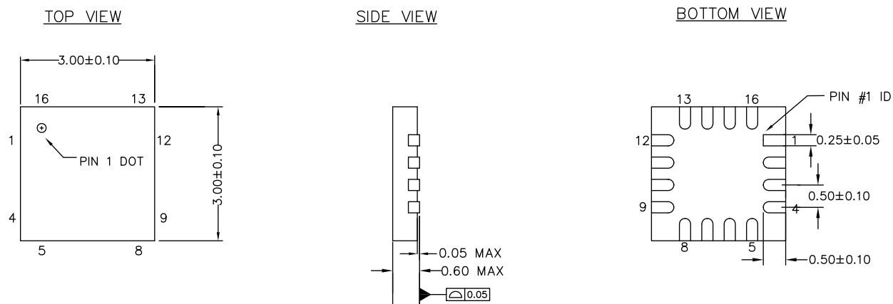
Figure 13. 16-pin Chip-On-Lead ( 3 \times 3 \times 0.6 mm) LG16A/LD16A (Sawn) Package Outline, 001-09116
