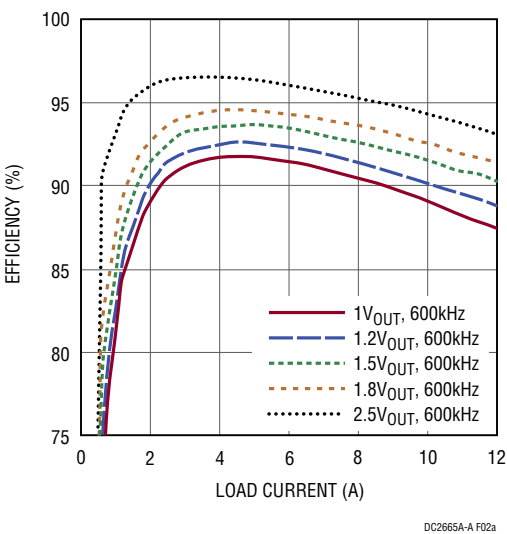
a) 3.3V IN CCM Efficiency vs Load Current
