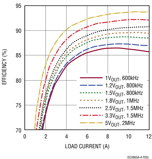
c) 12V IN CCM Efficiency vs Load Current
