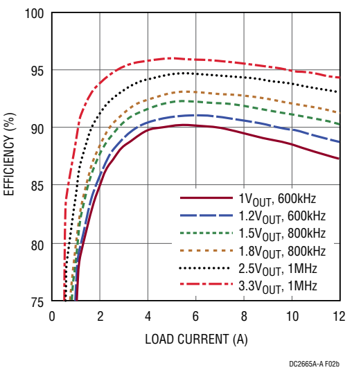
b) 5V IN CCM Efficiency vs Load Current
