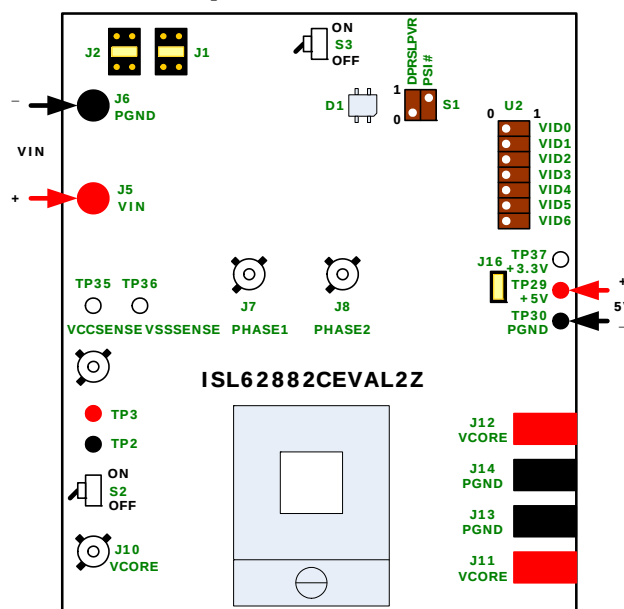
FIGURE 1. TEST SET-UP
