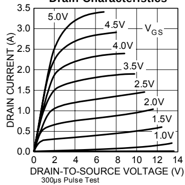
Drain Characteristics
