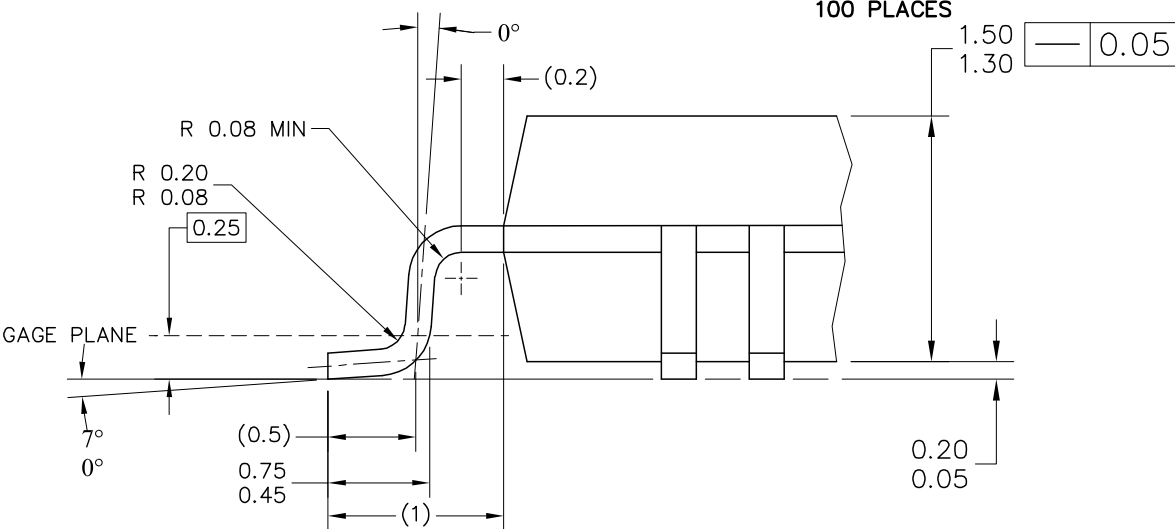
VIEW A
