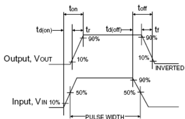
Switchin Waveforms
