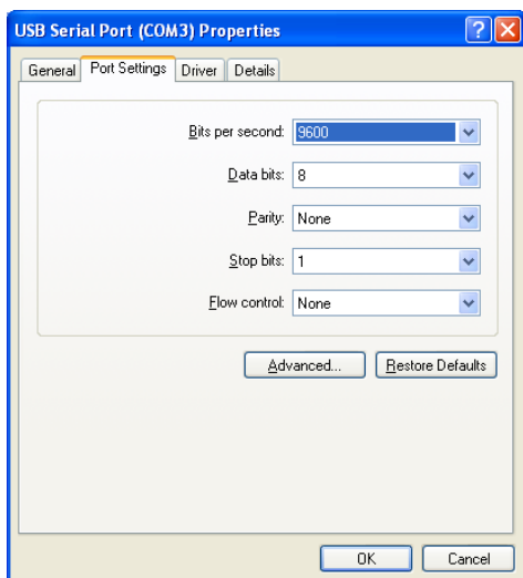
Figure 3-5 Settings Tab
