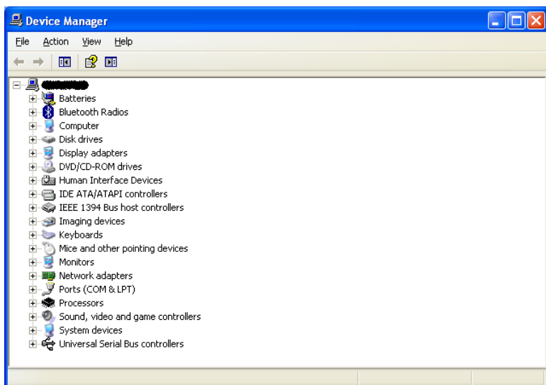
Figure 3-2 Device Manager
