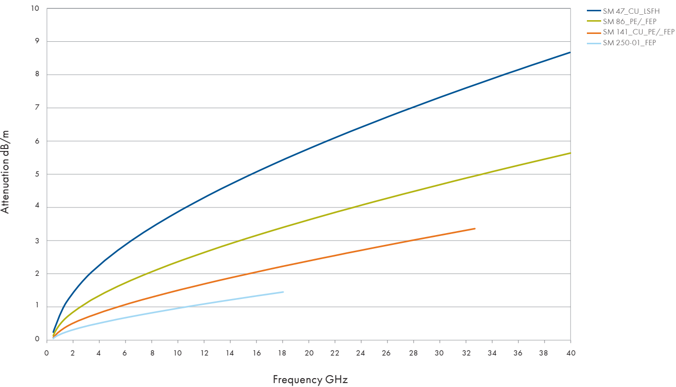
Attenuation (nominal values at +25 °C ambient temperature)
