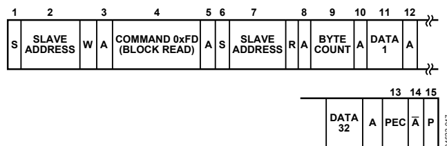
Figure 42. Block Read from the EEPROM or RAM with PEC
