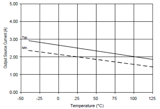
Figure 24A. Output Source Current vs. Temperature
