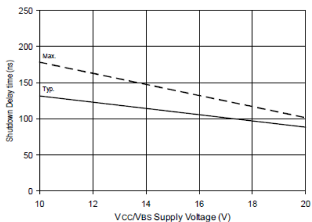
Figure 7B. Shutdown Time vs. V_{CC}/V_{BS} Supply Voltage
