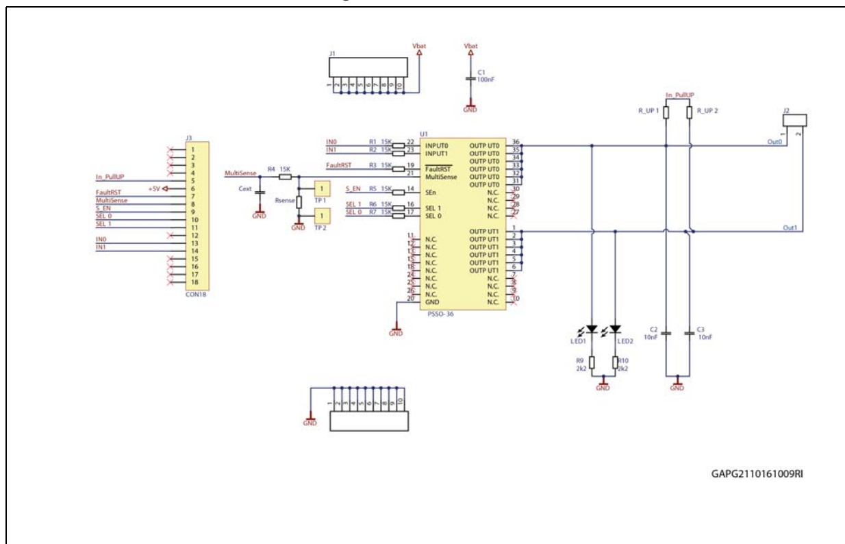
Figure 1. EV-VND7004AY schematic
